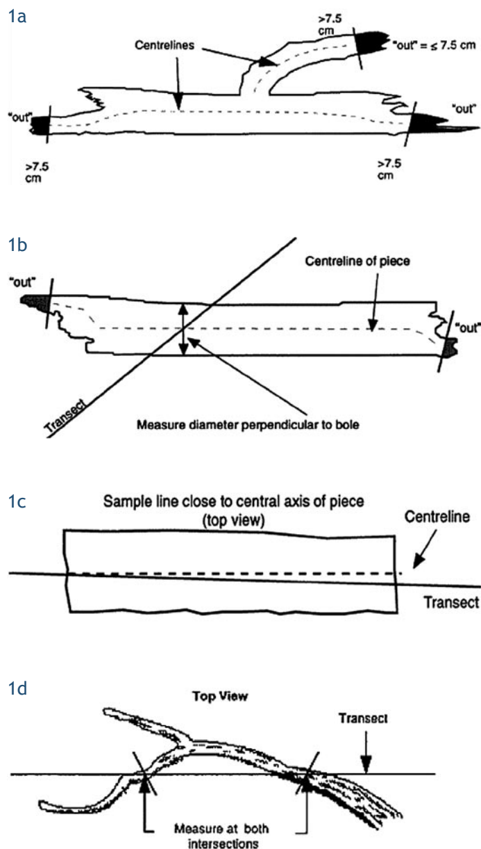
Figure A4-1. Rules for sampling CWD.
