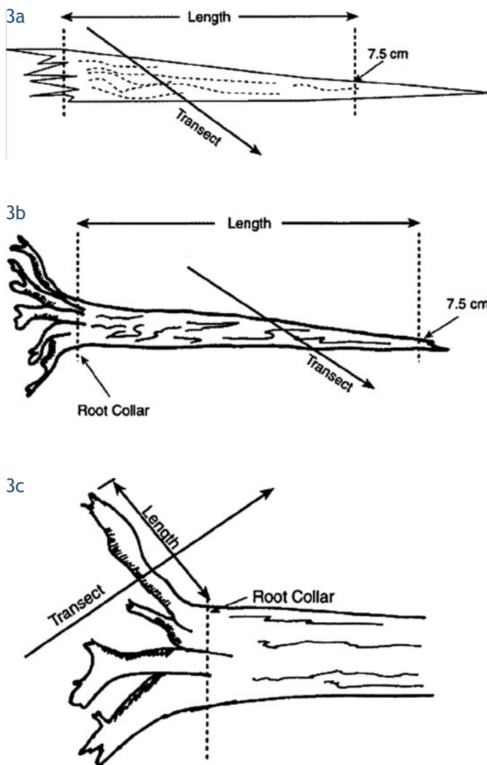
Figure A4-3. Rules for measuring length of CWD.
